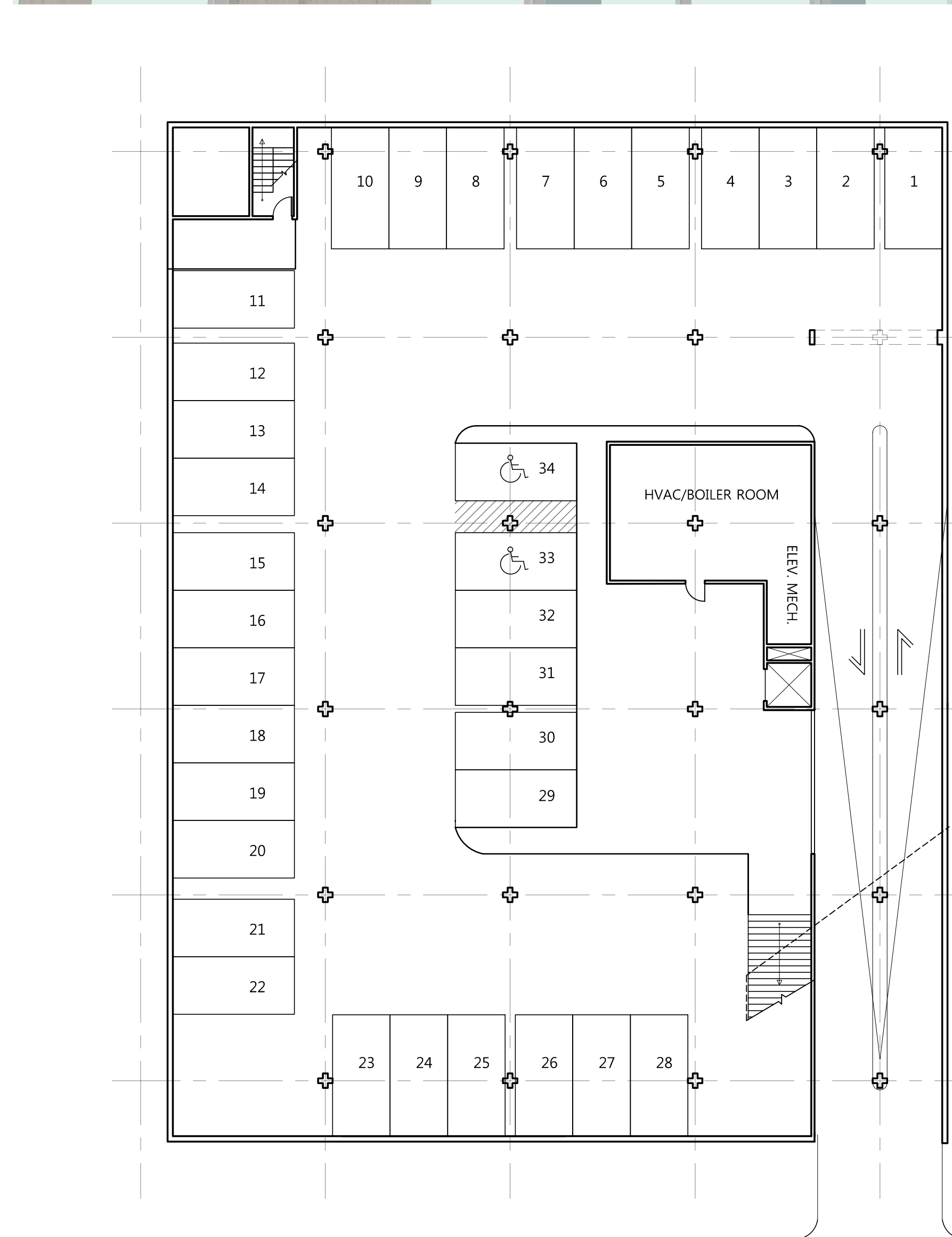
PLANS (1/16" = 1'-0")
